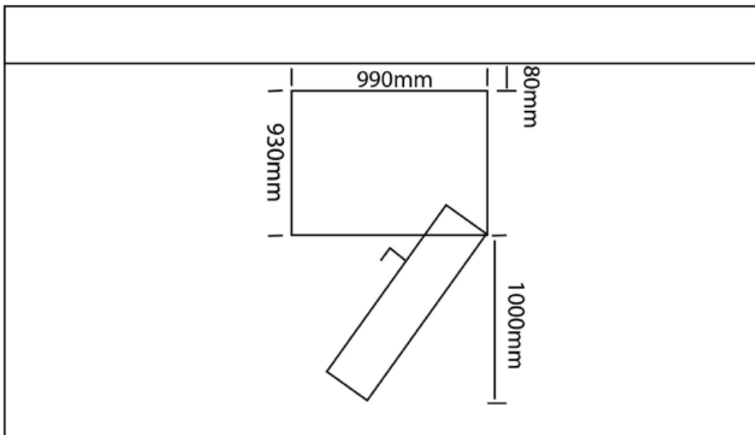
Diagram 2 (no cavity) against wall
